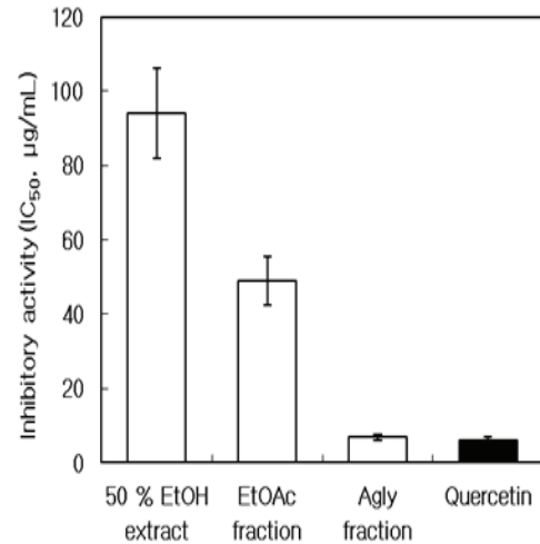
Fig. 6. The inhibitory effects of extract and fractions obtained from S. commixta twig and references compound on elastase
