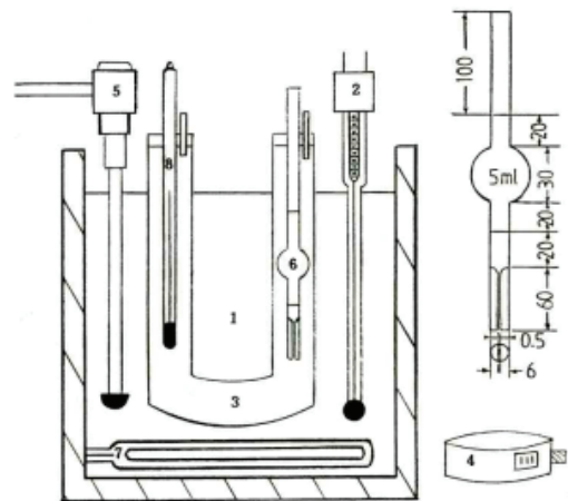
Fig. 1. Stalagmometer for the determination of the surface tension[3].
