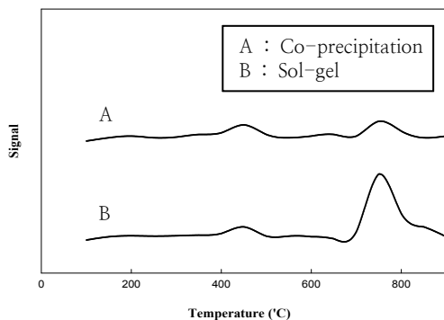
Fig. 6. O 2 -TPD curves for Mo-Bi-Cr-Si mixed oxide catalysts prepared by co-precipitation and sol-gel methods.
