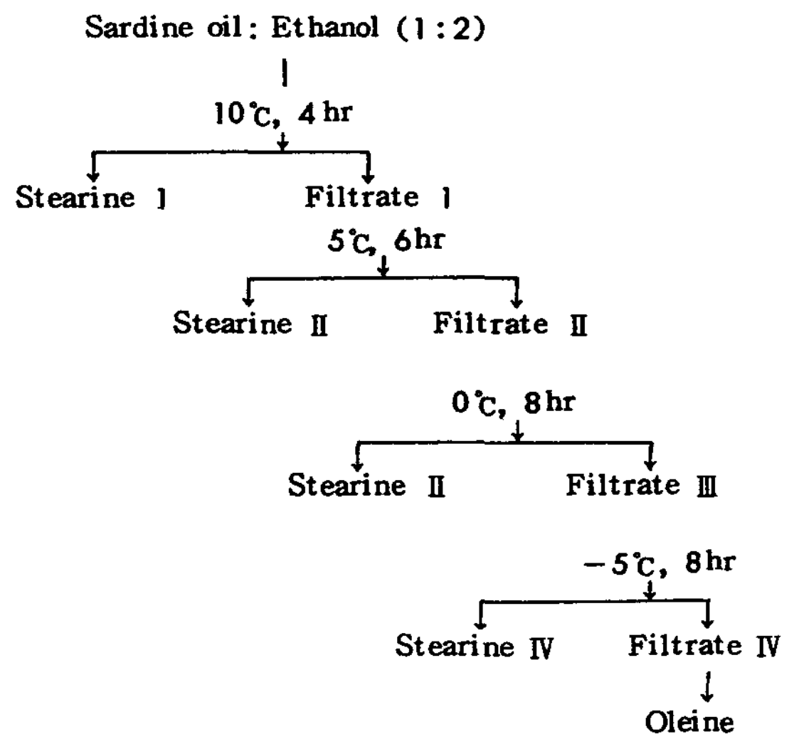
Fig. 2. Ethanol fractionation of sardine oil.
